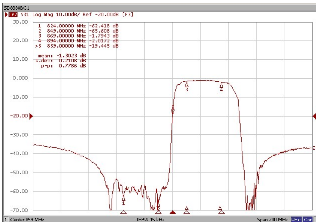
Rx Characteristic
